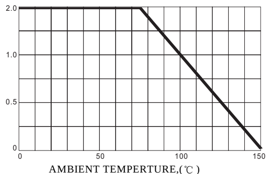
FIG.1 MAXIMUM AVERAGE FORWARD CURRENT DERATING
