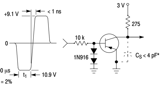
Figure 2. Storage and Fall Time Equivalent Test Circuit
